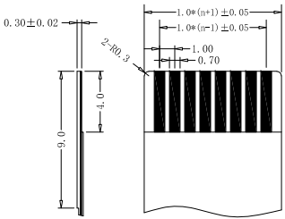
RECOMMENDED FPC/FFC DIMENSION
