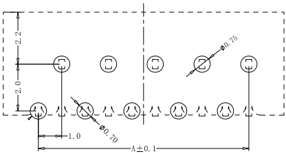
RECOMMENDED P.C.B LAYOUT GENERAL TOLERANCE:±0.05MM
